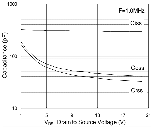
Fig.7 Capacitance
