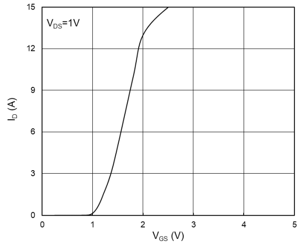
Fig.13 Transfer Characteristics
