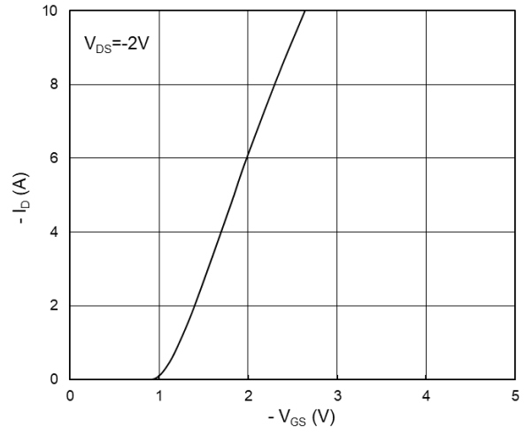
Fig.13 Transfer Characteristics
