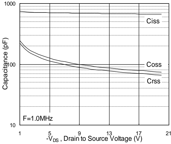
Fig.7 Capacitance
